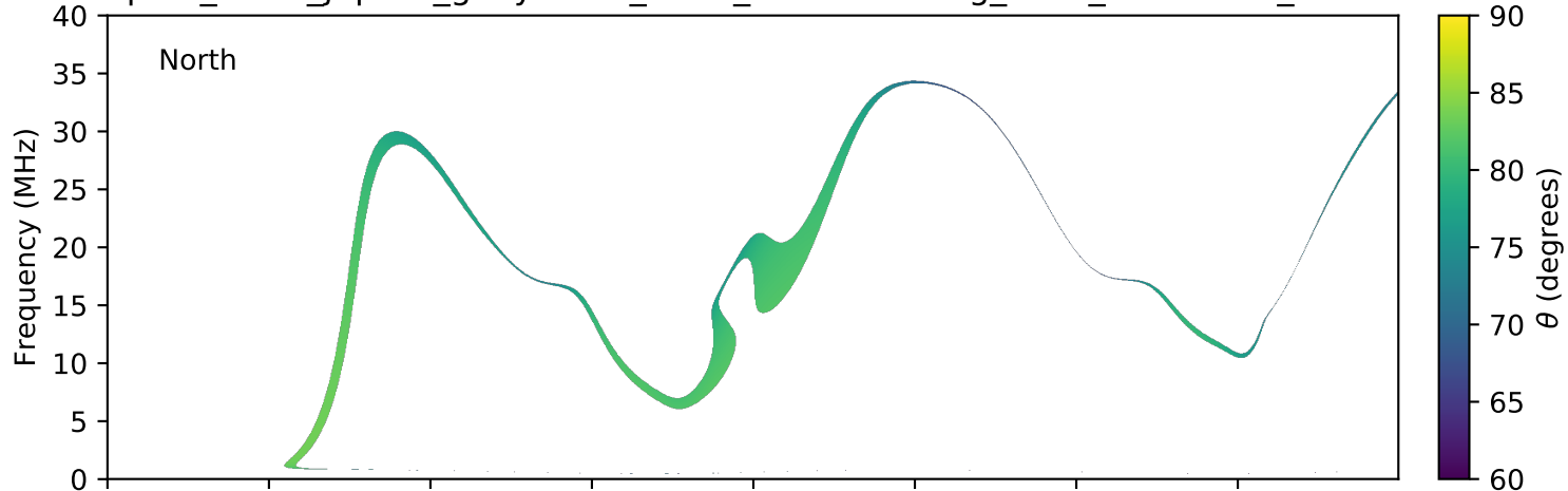
expres_earth_jupiter_ganymede_isaac_lossc-wid1deg_3kev_20170813_v01.cdf
