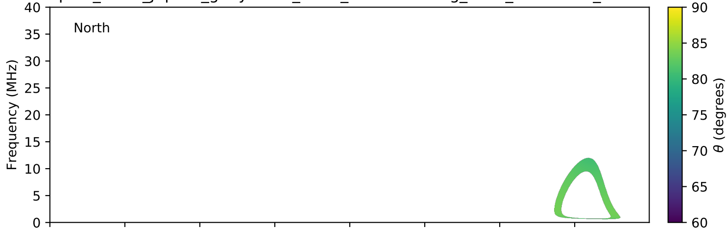
expres_earth_jupiter_ganymede_isaac_lossc-wid1deg_3kev_20170812_v01.cdf
