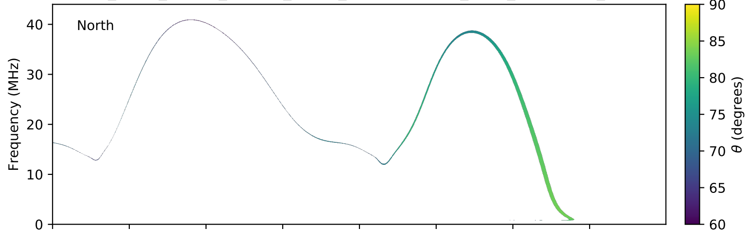
expres_earth_jupiter_europa_jrm09_lossc-wid1deg_3kev_20170830_v01.cdf
