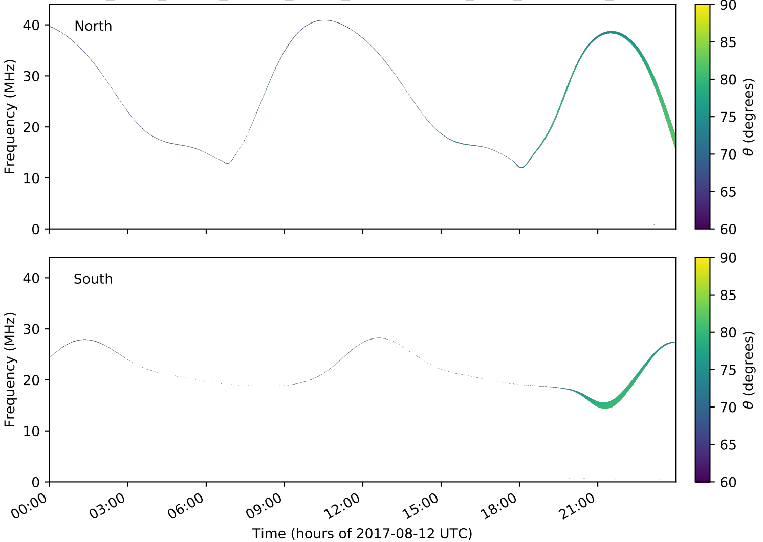
expres_earth_jupiter_europa_jrm09_lossc-wid1deg_3kev_20170812_v01.cdf
