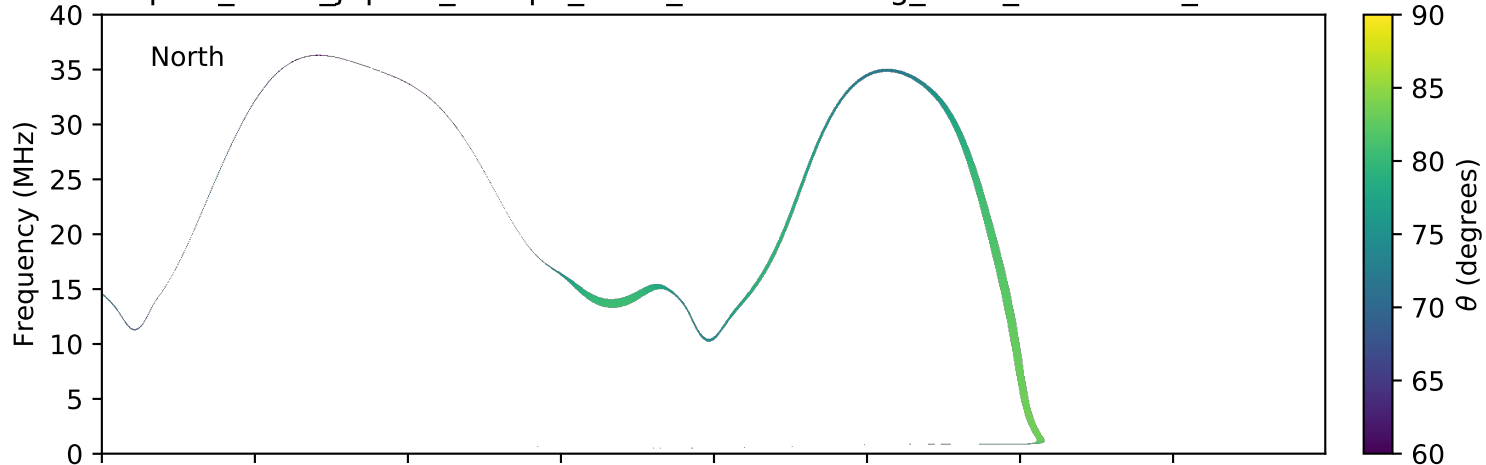
expres_earth_jupiter_europa_isaac_lossc-wid1deg_3kev_20170823_v01.cdf
