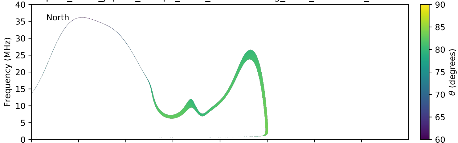
expres_earth_jupiter_europa_isaac_lossc-wid1deg_3kev_20170809_v01.cdf
