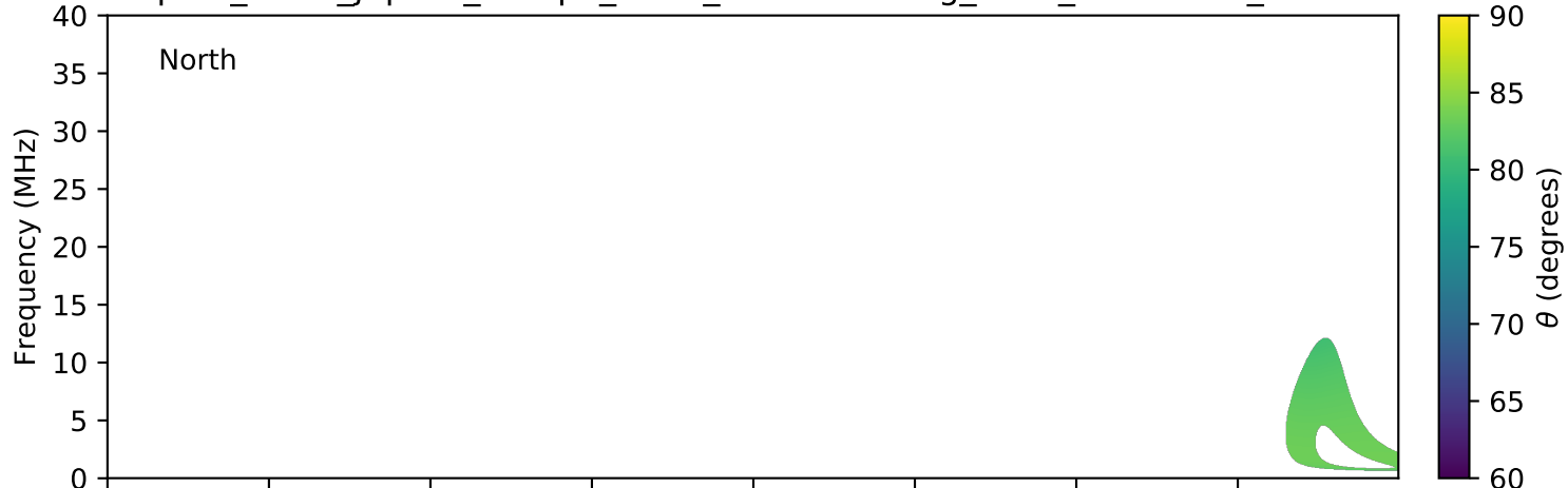
expres_earth_jupiter_europa_isaac_lossc-wid1deg_3kev_20170807_v01.cdf
