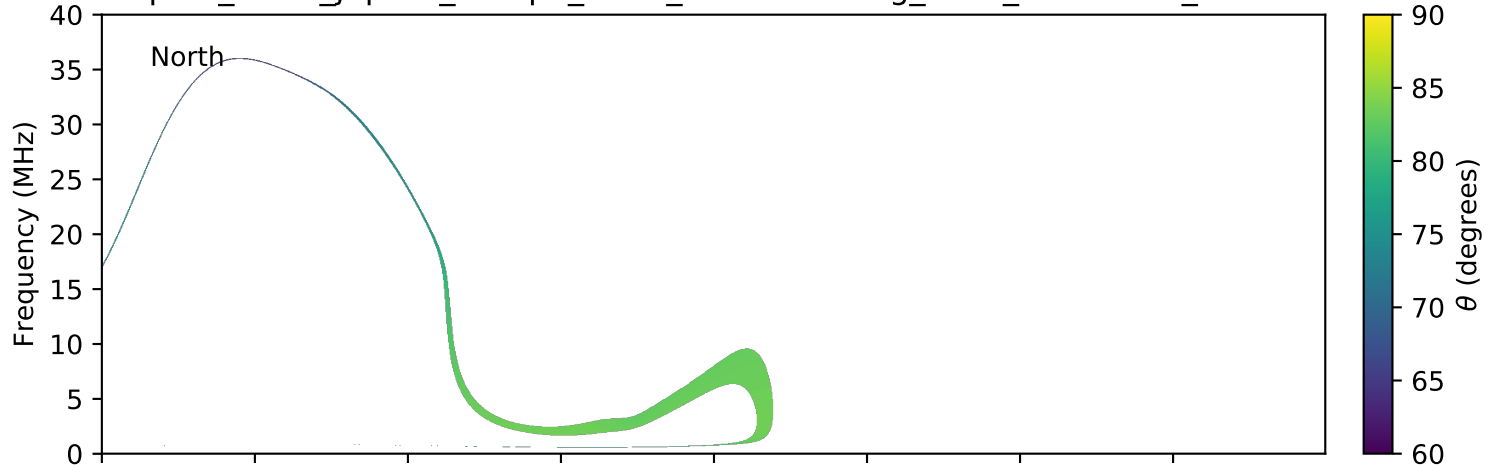
expres_earth_jupiter_europa_isaac_lossc-wid1deg_3kev_20170802_v01.cdf
