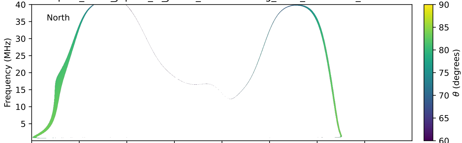
expres_earth_jupiter_io_jrm33_lossc-wid1deg_3kev_20170725_v11.cdf
