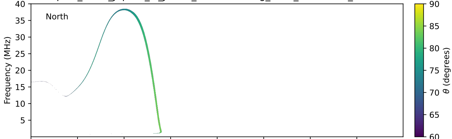
expres_earth_jupiter_io_jrm33_lossc-wid1deg_3kev_20170706_v11.cdf
