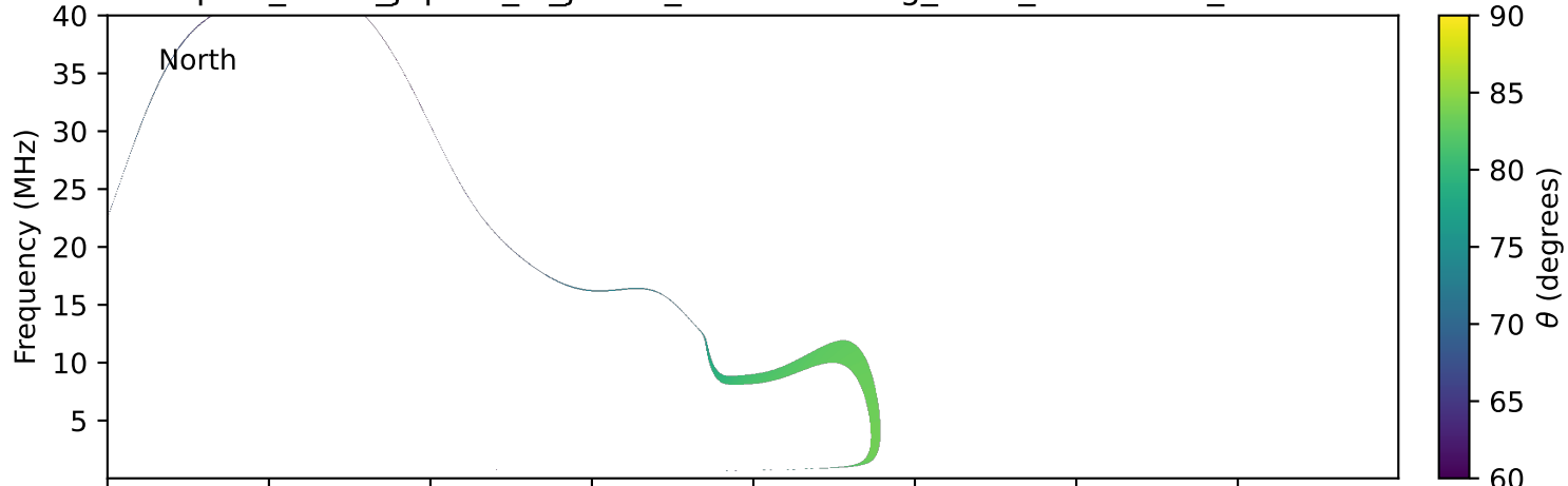
expres_earth_jupiter_io_jrm33_lossc-wid1deg_3kev_20170704_v11.cdf
