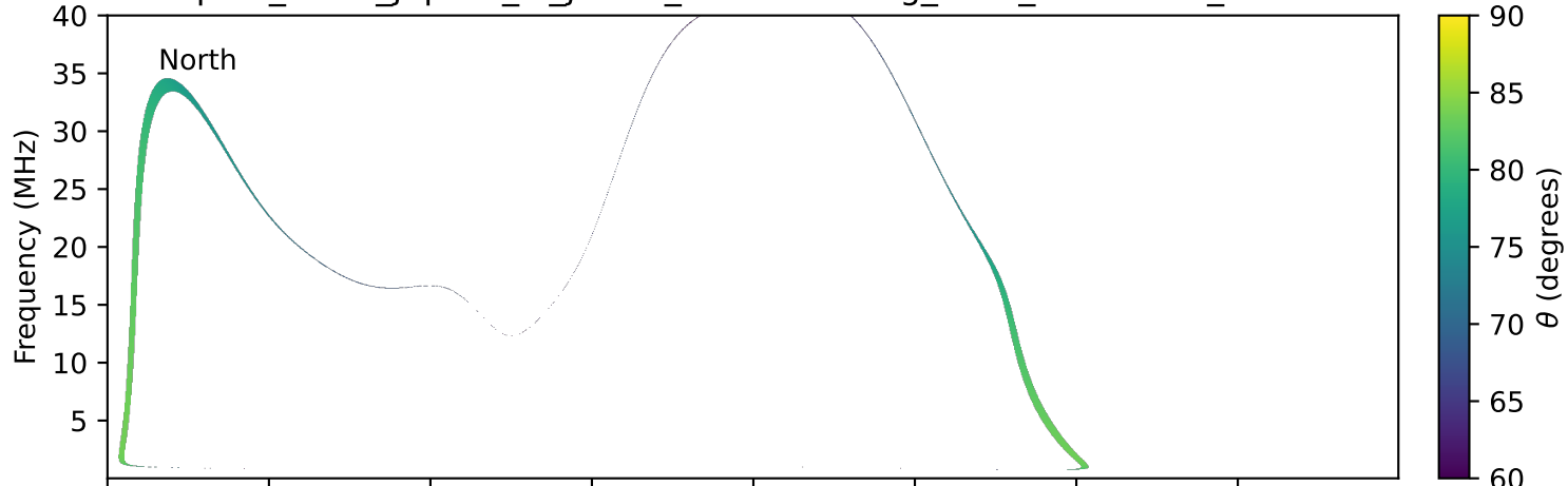
expres_earth_jupiter_io_jrm33_lossc-wid1deg_3kev_20170702_v11.cdf
