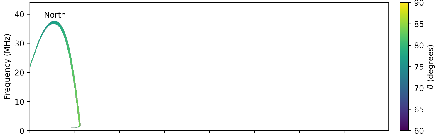
expres_earth_jupiter_io_jrm09_lossc-wid1deg_3kev_20170731_v01.cdf
