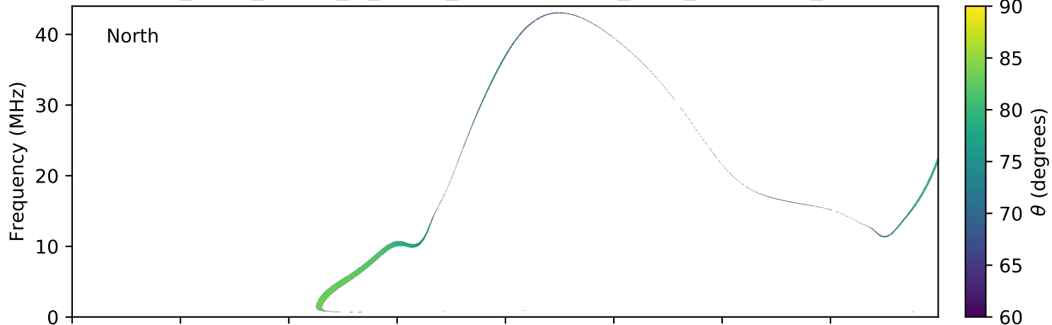
expres_earth_jupiter_io_jrm09_lossc-wid1deg_3kev_20170730_v01.cdf
