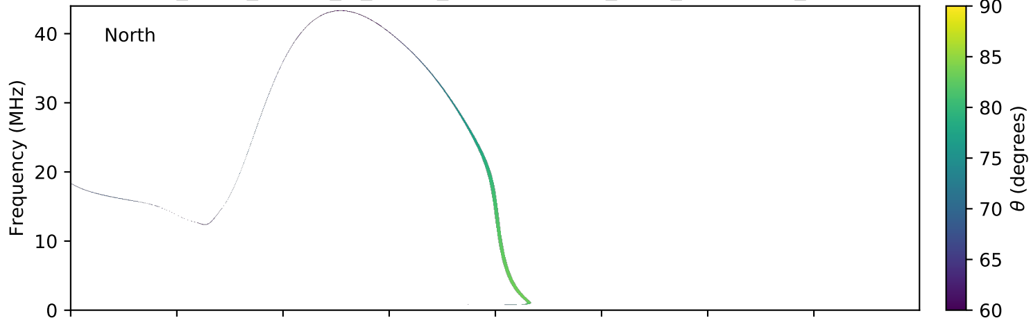
expres_earth_jupiter_io_jrm09_lossc-wid1deg_3kev_20170727_v01.cdf
