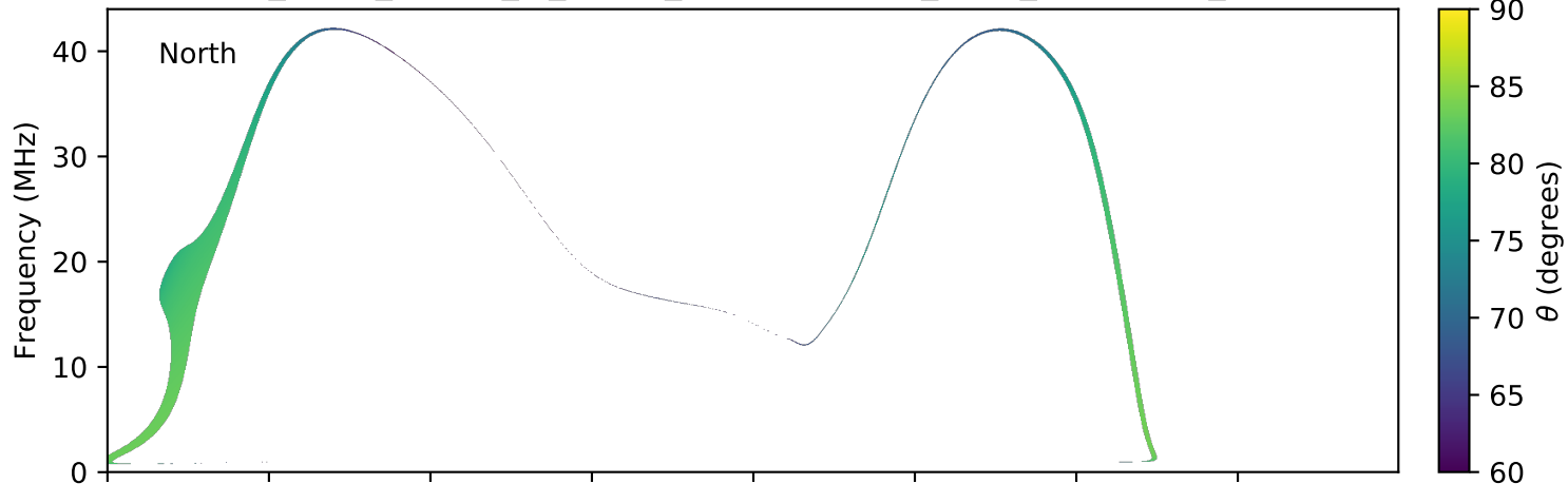
expres_earth_jupiter_io_jrm09_lossc-wid1deg_3kev_20170725_v01.cdf
