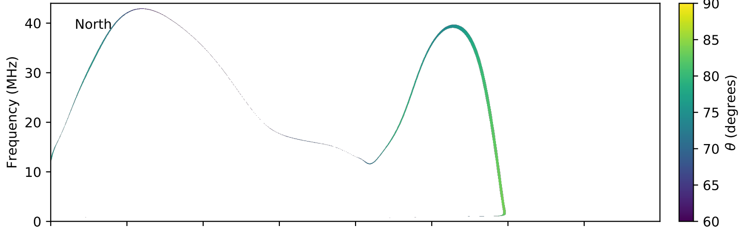
expres_earth_jupiter_io_jrm09_lossc-wid1deg_3kev_20170718_v01.cdf
