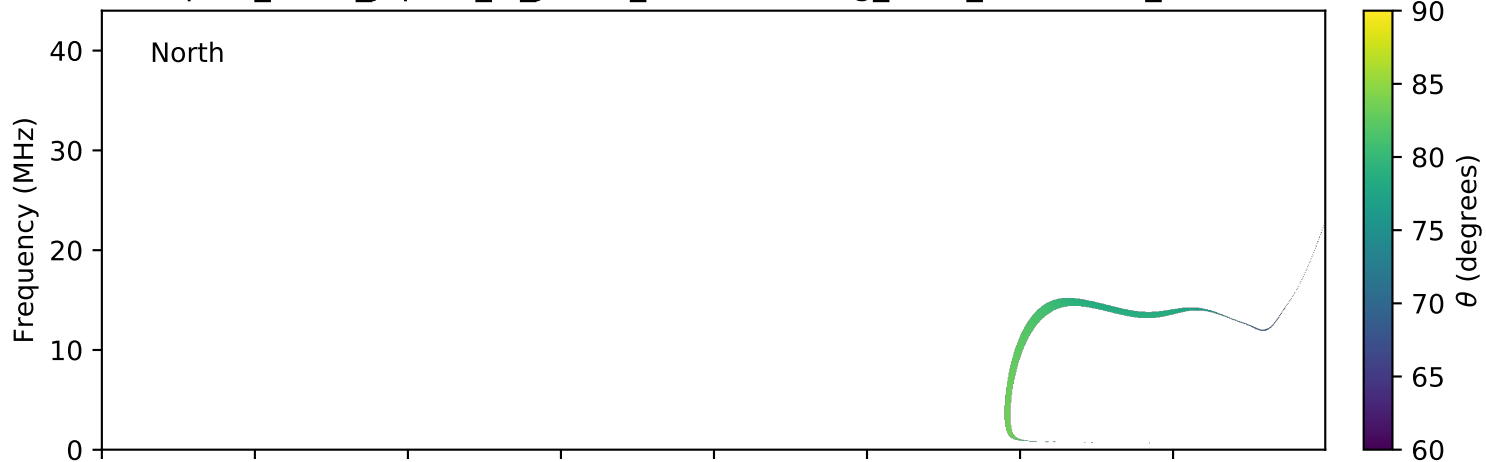
expres_earth_jupiter_io_jrm09_lossc-wid1deg_3kev_20170703_v01.cdf
