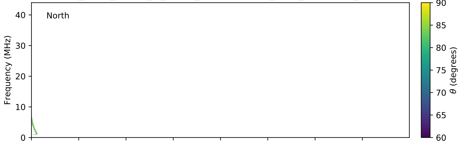
expres_earth_jupiter_io_jrm09_lossc-wid1deg_3kev_20170701_v01.cdf
