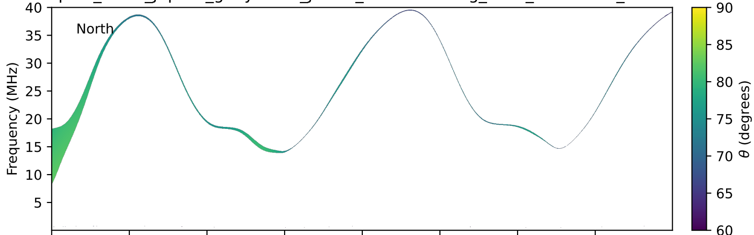
expres_earth_jupiter_ganymede_jrm33_lossc-wid1deg_3kev_20170723_v11.cdf
