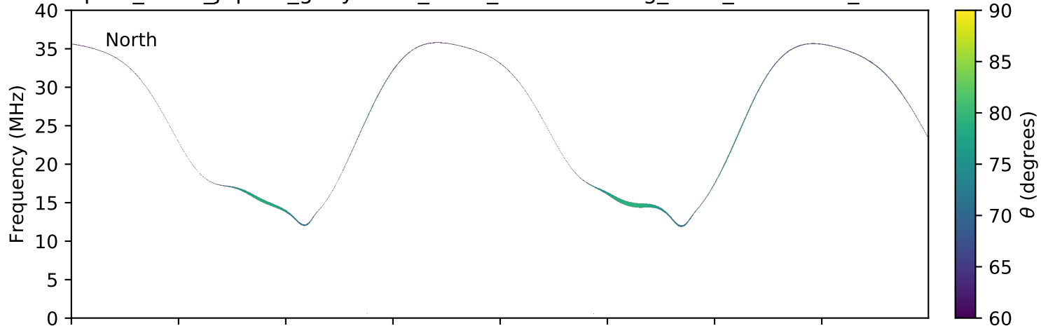
expres_earth_jupiter_ganymede_isaac_lossc-wid1deg_3kev_20170731_v01.cdf
