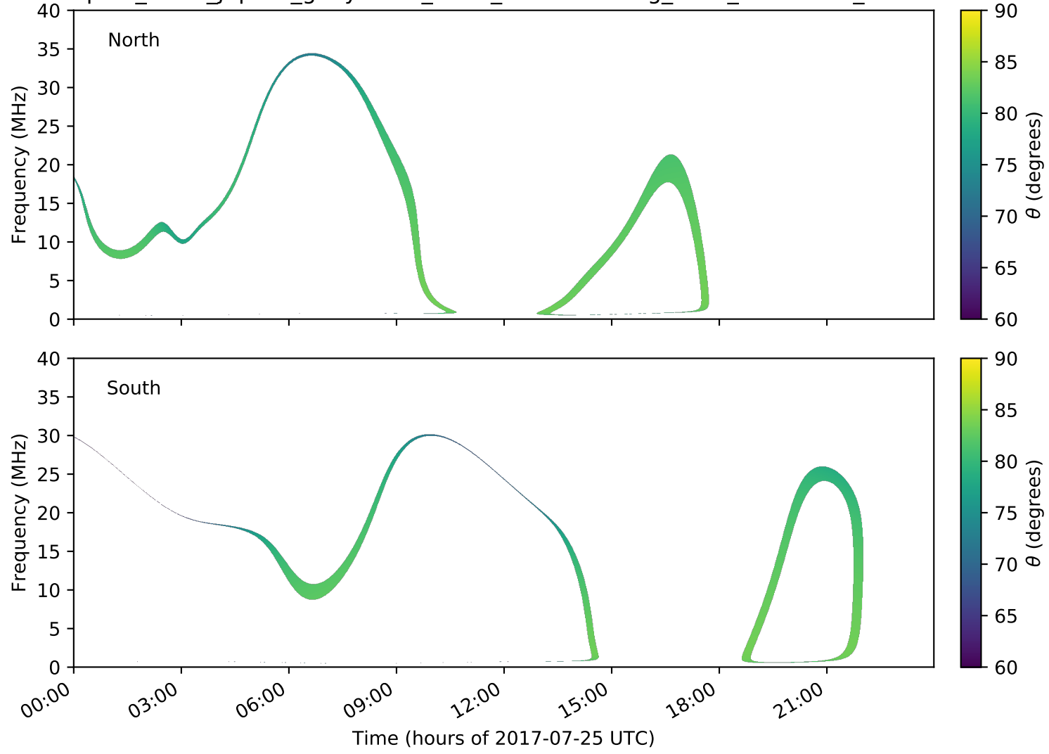
expres_earth_jupiter_ganymede_isaac_lossc-wid1deg_3kev_20170725_v01.cdf
