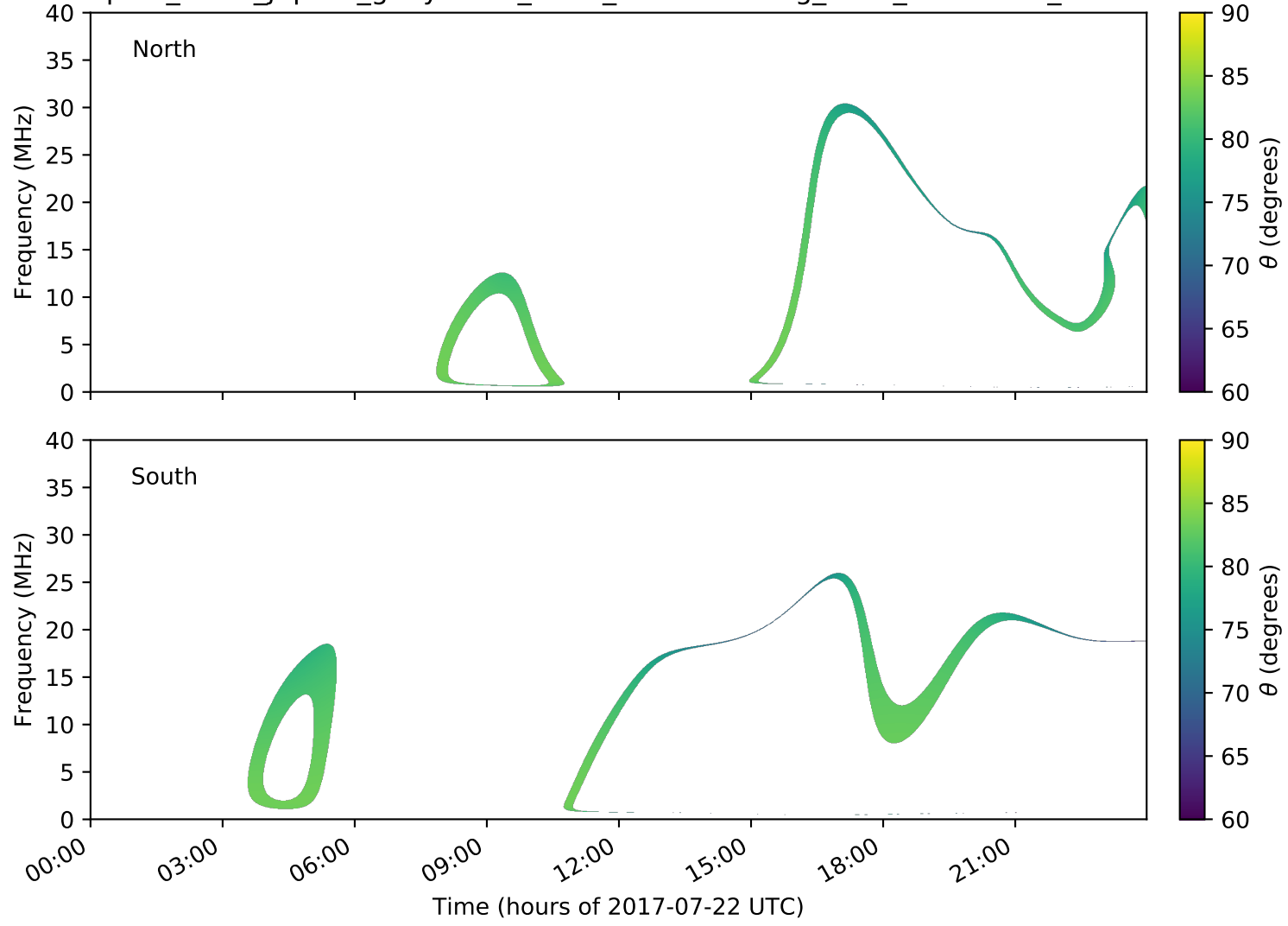
expres_earth_jupiter_ganymede_isaac_lossc-wid1deg_3kev_20170722_v01.cdf
