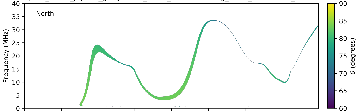
expres_earth_jupiter_ganymede_isaac_lossc-wid1deg_3kev_20170708_v01.cdf
