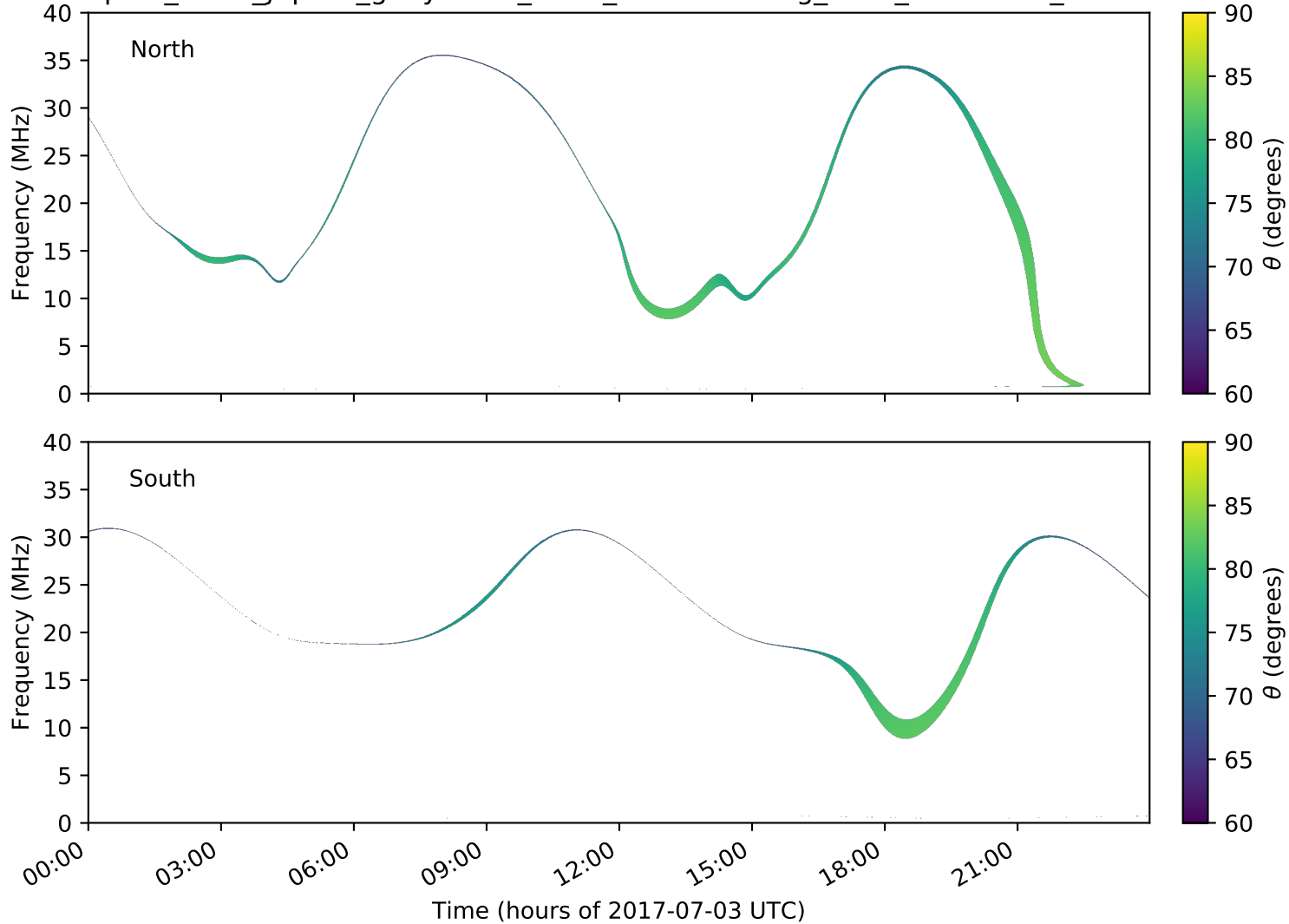
expres_earth_jupiter_ganymede_isaac_lossc-wid1deg_3kev_20170703_v01.cdf
