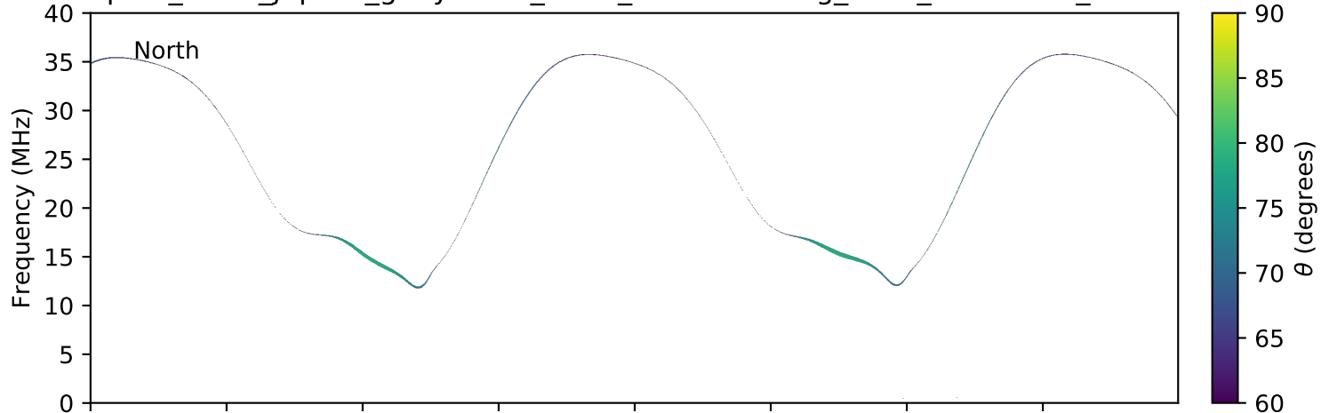
expres_earth_jupiter_ganymede_isaac_lossc-wid1deg_3kev_20170702_v01.cdf
