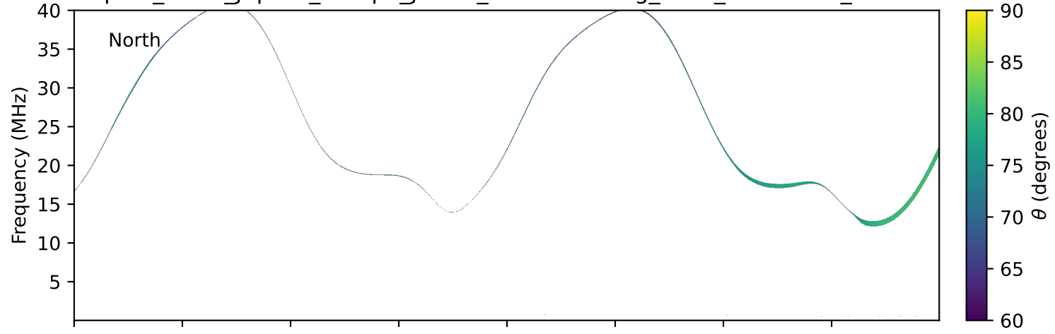
expres_earth_jupiter_europa_jrm33_lossc-wid1deg_3kev_20170711_v11.cdf
