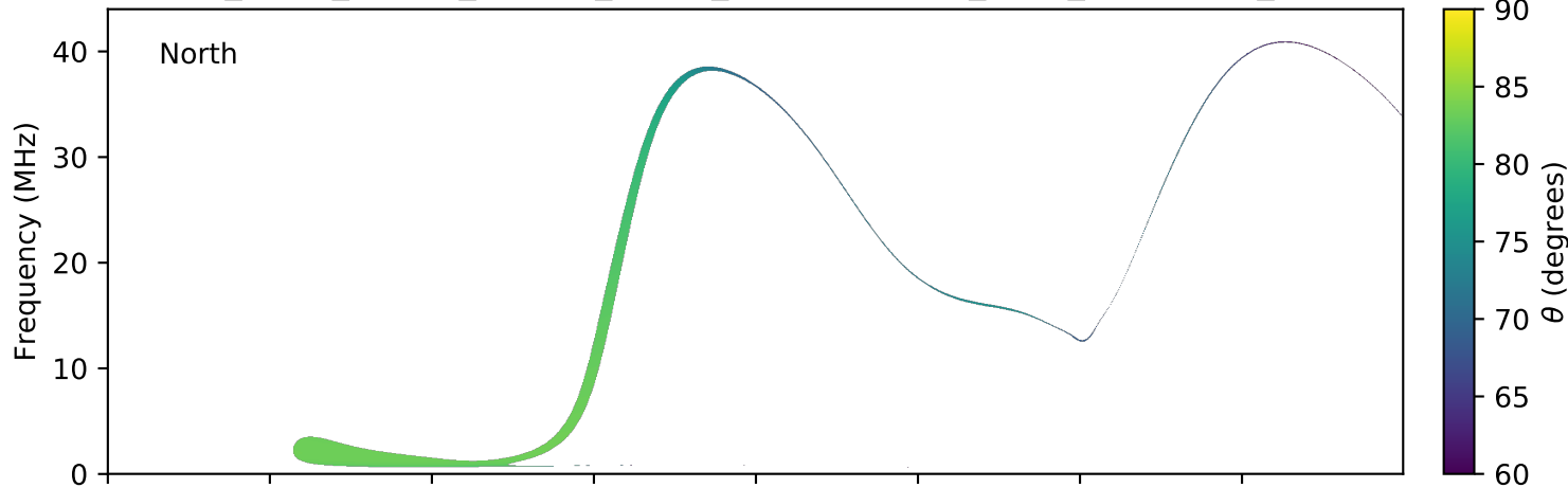
expres_earth_jupiter_europa_jrm09_lossc-wid1deg_3kev_20170721_v01.cdf
