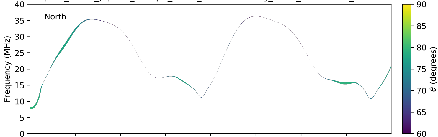
expres_earth_jupiter_europa_isaac_lossc-wid1deg_3kev_20170725_v01.cdf
