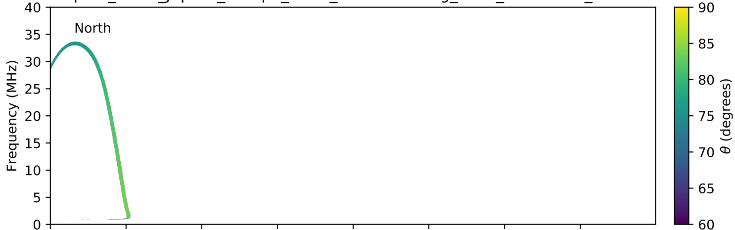
expres_earth_jupiter_europa_isaac_lossc-wid1deg_3kev_20170712_v01.cdf
