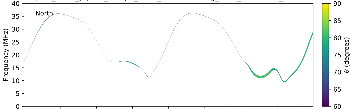
expres_earth_jupiter_europa_isaac_lossc-wid1deg_3kev_20170711_v01.cdf
