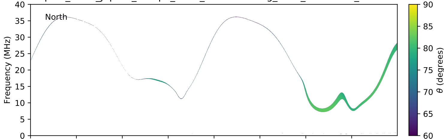
expres_earth_jupiter_europa_isaac_lossc-wid1deg_3kev_20170704_v01.cdf
