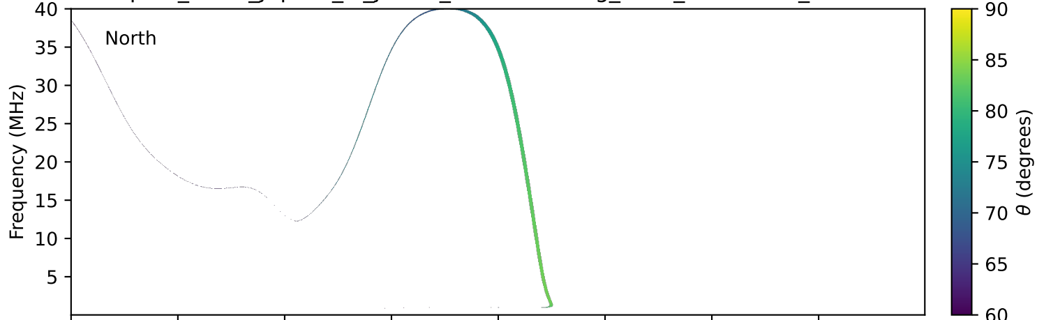
expres_earth_jupiter_io_jrm33_lossc-wid1deg_3kev_20170611_v11.cdf
