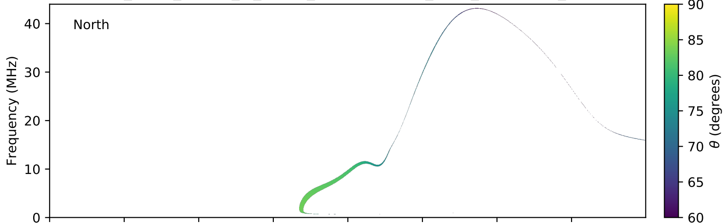
expres_earth_jupiter_io_jrm09_lossc-wid1deg_3kev_20170628_v01.cdf
