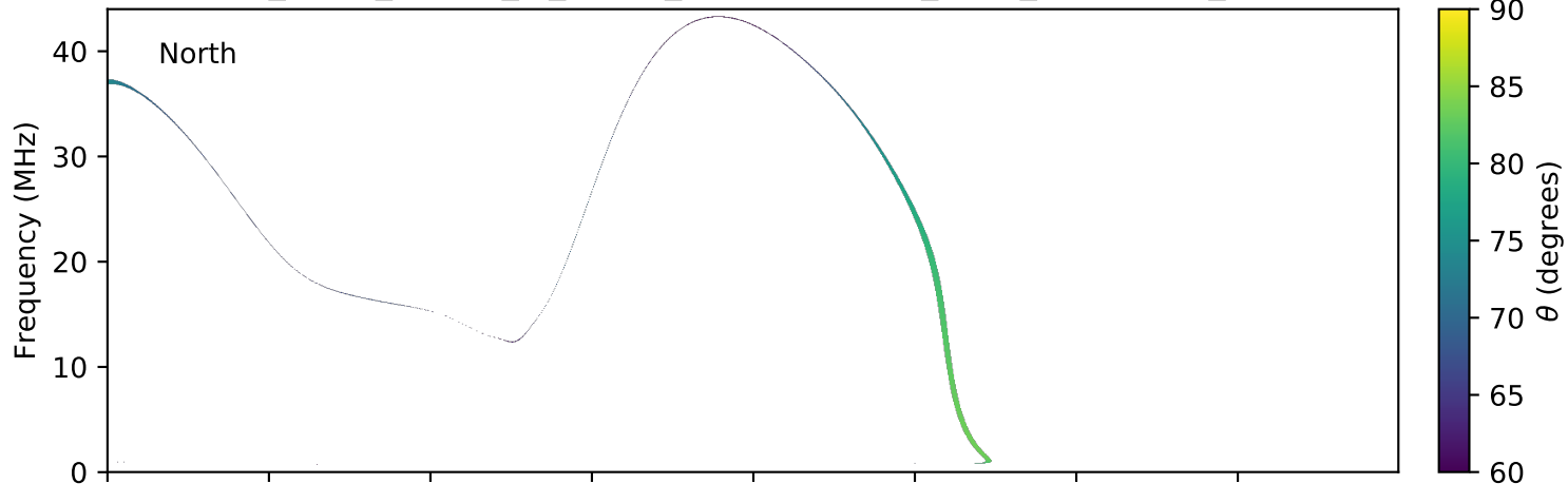
expres_earth_jupiter_io_jrm09_lossc-wid1deg_3kev_20170625_v01.cdf
