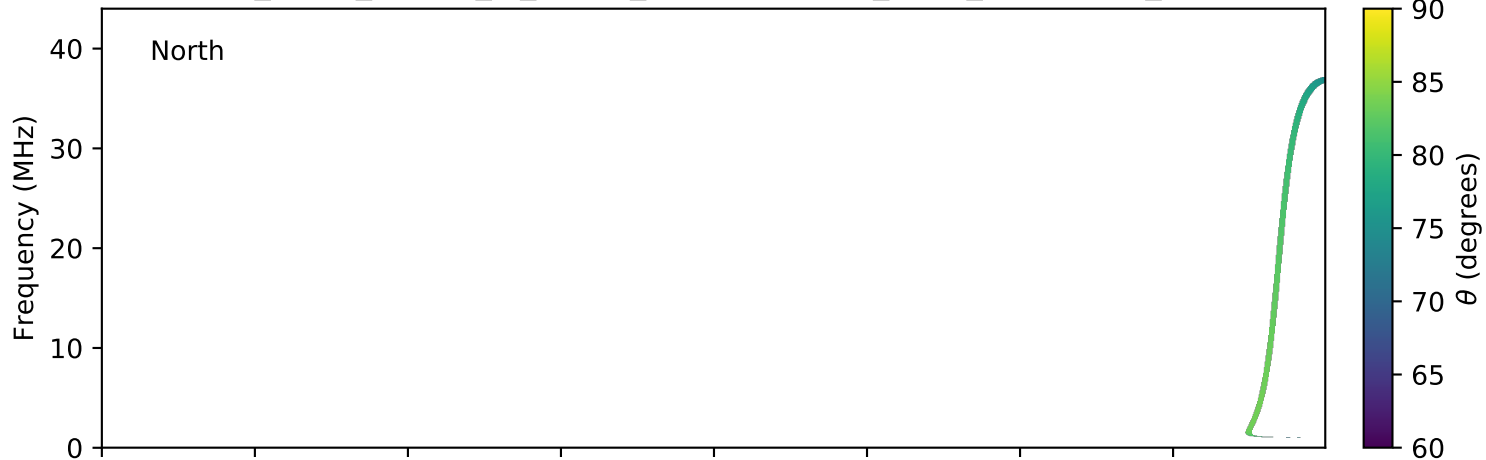
expres_earth_jupiter_io_jrm09_lossc-wid1deg_3kev_20170624_v01.cdf
