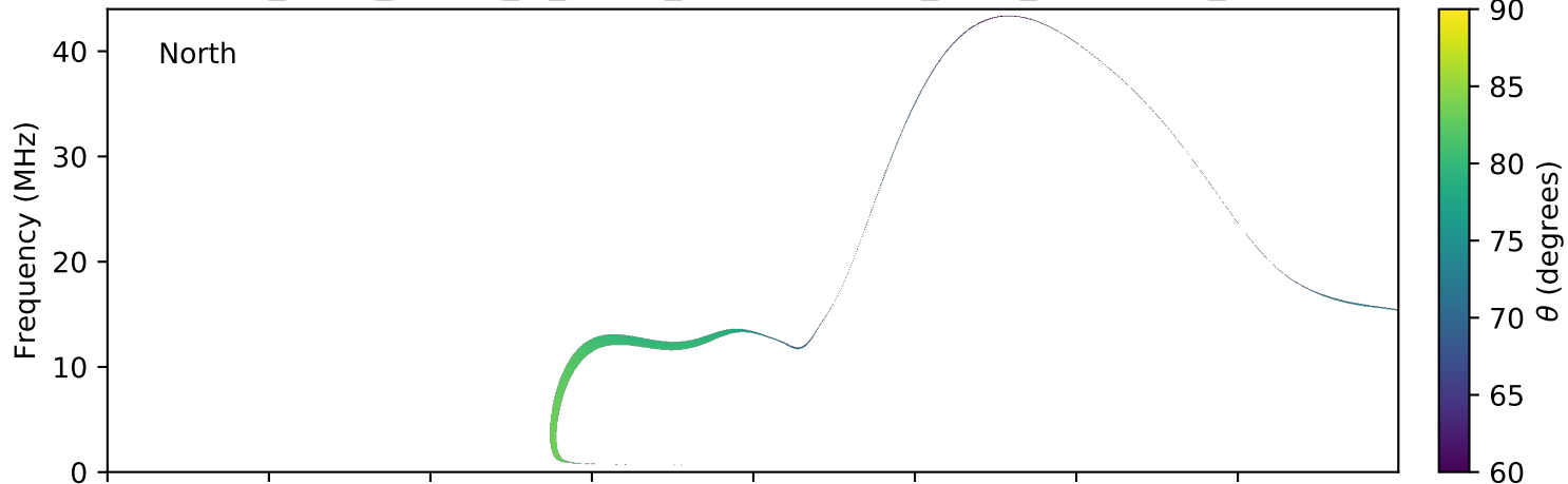
expres_earth_jupiter_io_jrm09_lossc-wid1deg_3kev_20170621_v01.cdf
