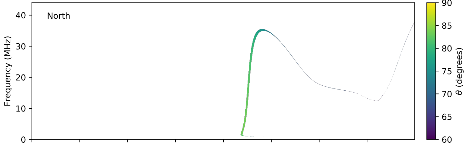
expres_earth_jupiter_io_jrm09_lossc-wid1deg_3kev_20170612_v01.cdf
