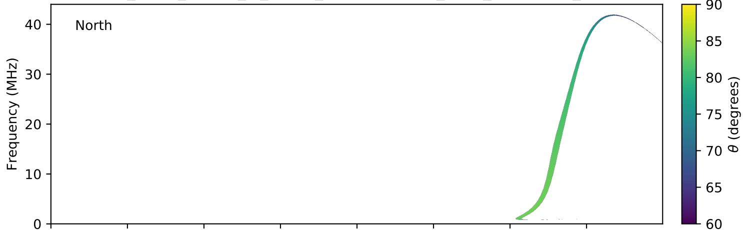
expres_earth_jupiter_io_jrm09_lossc-wid1deg_3kev_20170610_v01.cdf
