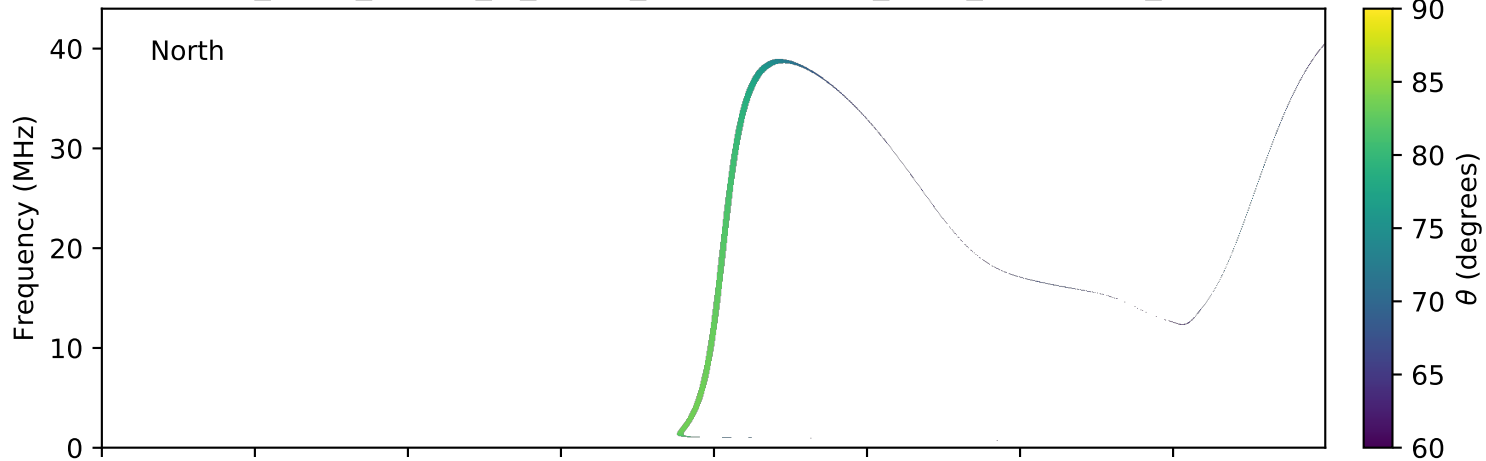
expres_earth_jupiter_io_jrm09_lossc-wid1deg_3kev_20170605_v01.cdf
