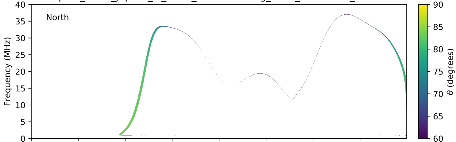
expres_earth_jupiter_io_isaac_lossc-wid1deg_3kev_20170630_v01.cdf
