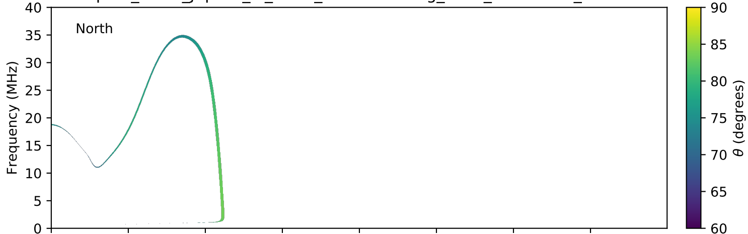
expres_earth_jupiter_io_isaac_lossc-wid1deg_3kev_20170629_v01.cdf
