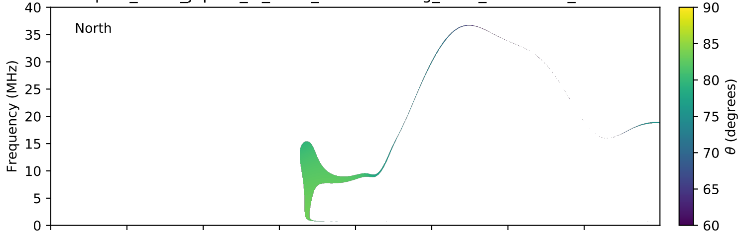
expres_earth_jupiter_io_isaac_lossc-wid1deg_3kev_20170628_v01.cdf
