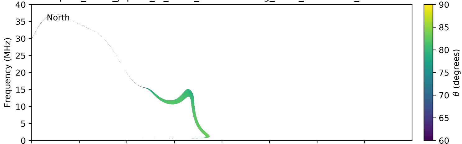
expres_earth_jupiter_io_isaac_lossc-wid1deg_3kev_20170627_v01.cdf
