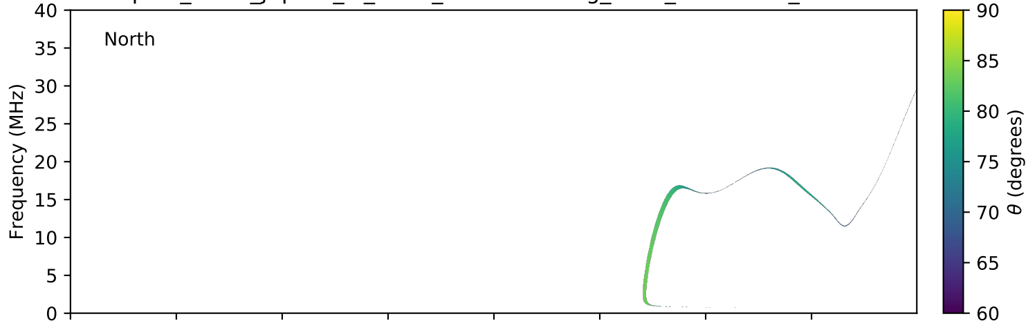
expres_earth_jupiter_io_isaac_lossc-wid1deg_3kev_20170626_v01.cdf
