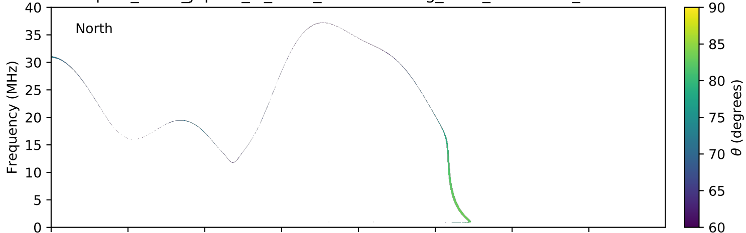
expres_earth_jupiter_io_isaac_lossc-wid1deg_3kev_20170625_v01.cdf
