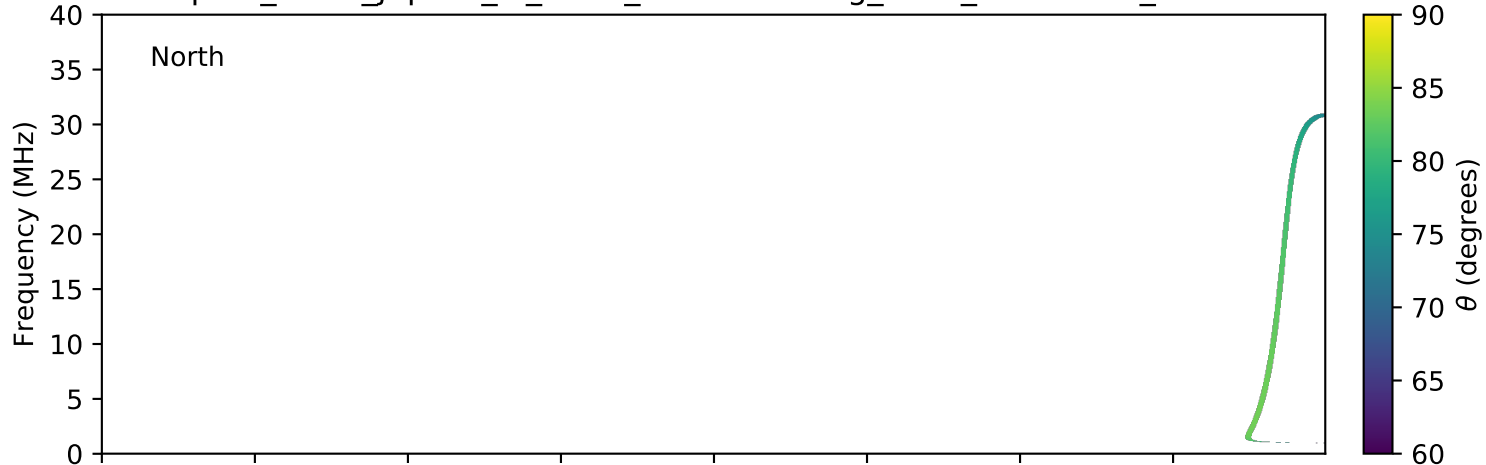
expres_earth_jupiter_io_isaac_lossc-wid1deg_3kev_20170624_v01.cdf
