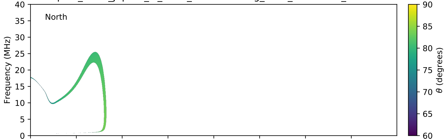
expres_earth_jupiter_io_isaac_lossc-wid1deg_3kev_20170622_v01.cdf
