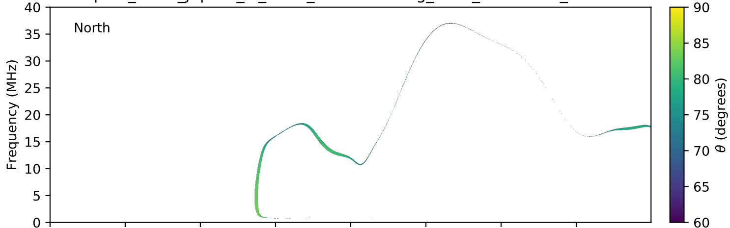
expres_earth_jupiter_io_isaac_lossc-wid1deg_3kev_20170621_v01.cdf
