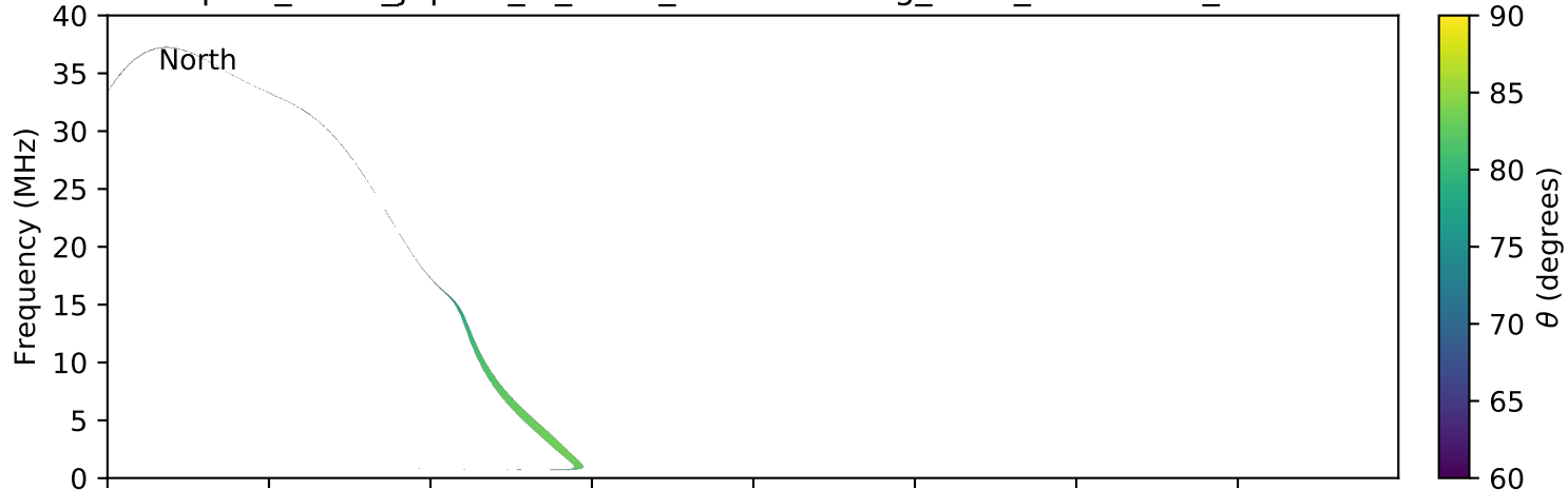
expres_earth_jupiter_io_isaac_lossc-wid1deg_3kev_20170620_v01.cdf
